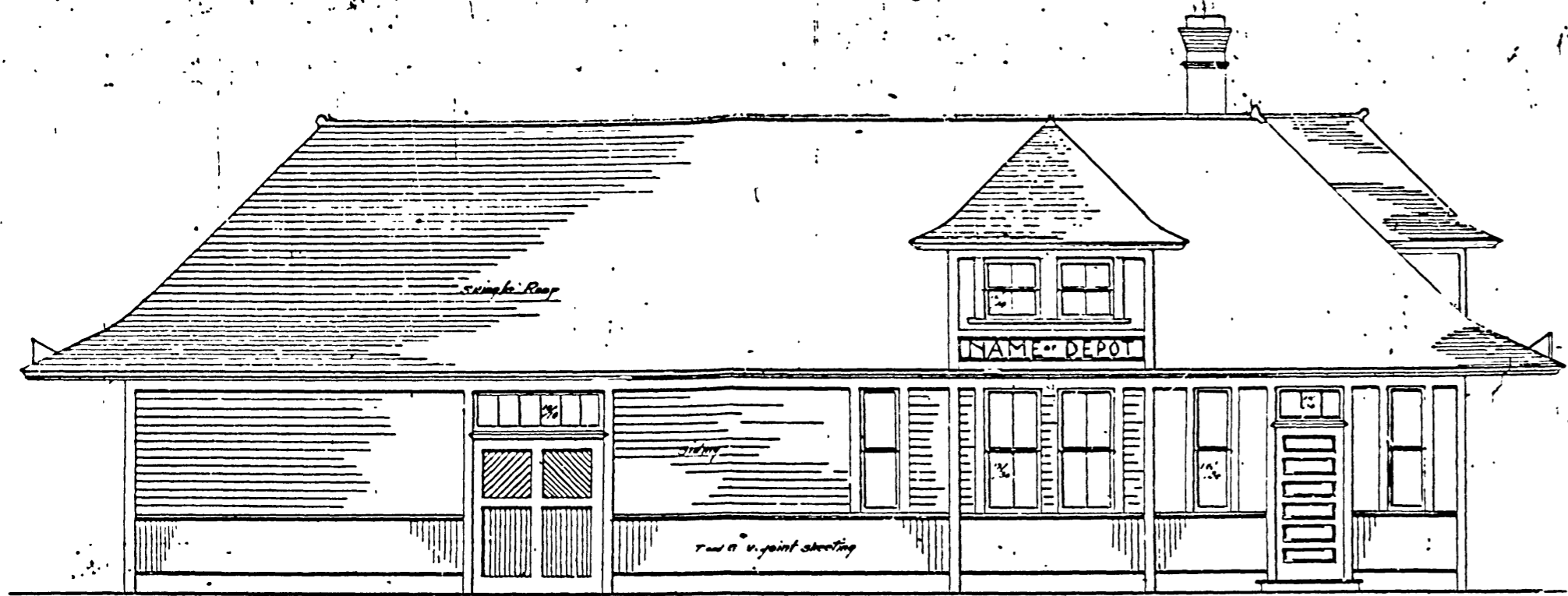
SOUTH ELEVATION
