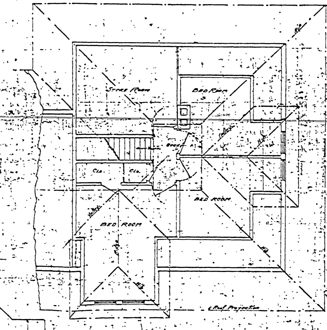
ATTIC & ROOF PLAN
